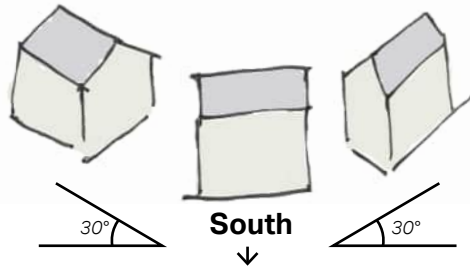
Building/roof orientation for solar gain
